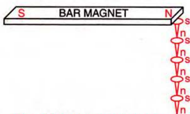
Fig. 10.3 Magnetic induction
