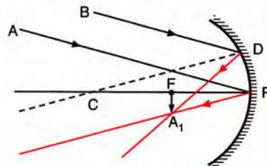
Fig. 7.32 When the object is at far distance
