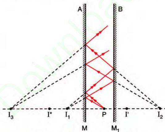
Fig. 7.18 Images formed in two parallel mirrors
