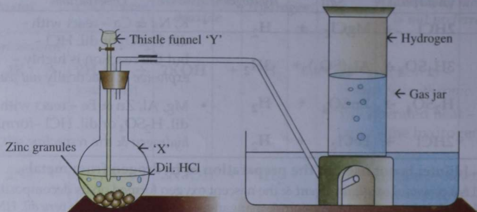
Laboratory preparation of hydrogen by action of dil. HCl on zinc.
