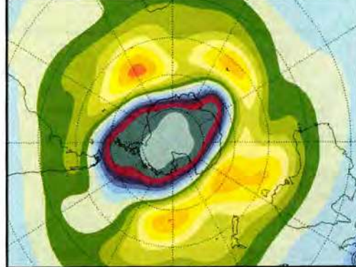
Fig. 10.5 Ozone hole — depletion
