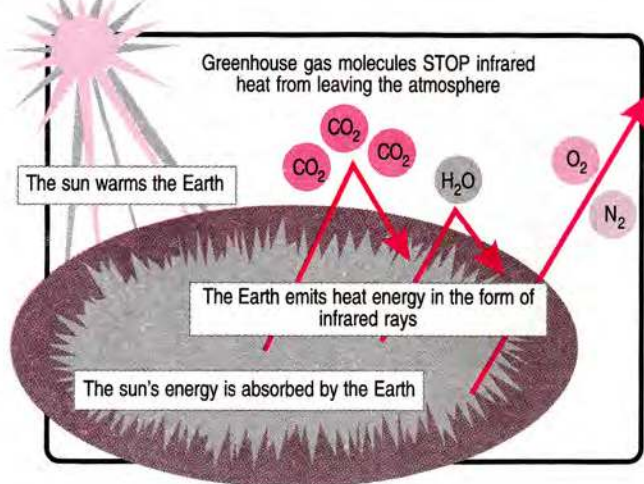
Fig. 8.4 Green House effect
