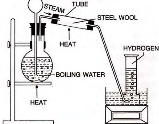
Fig. 6.5 Action of iron on steam
