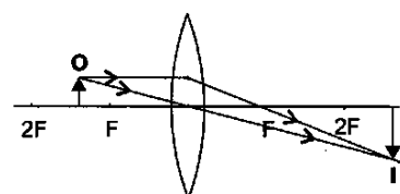
Fig. 2.17 Object anywhere between 2F and F
