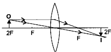
Fig. 2.16 Object at 2F
