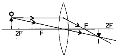
Fig. 2.15 Object beyond 2F but not infinity
