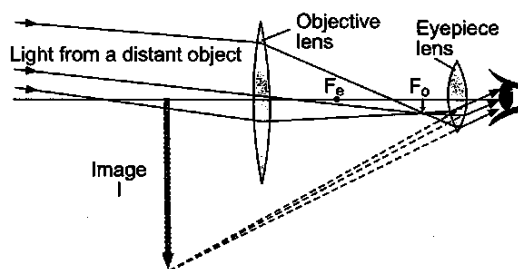
Fig. 2.27 Image formed in a telescope
