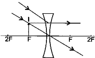
Fig. 2.20 Object at infinity
