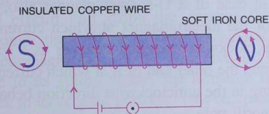
Fig. 13.2 Bar electromagnet
