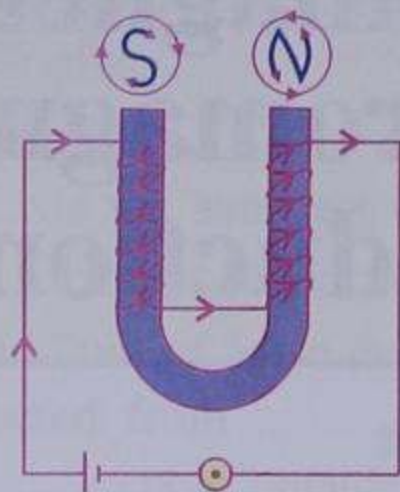
Fig. 13.3 U-shaped electromagnet
