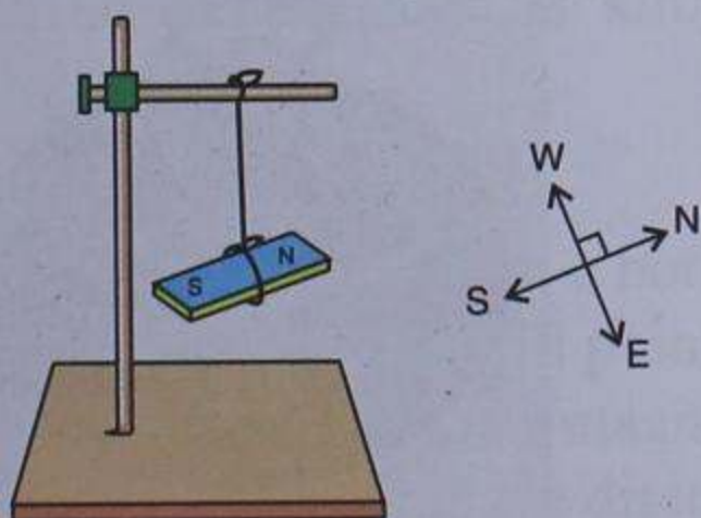
Fig. 12.3 A magnet always takes north-south direction
