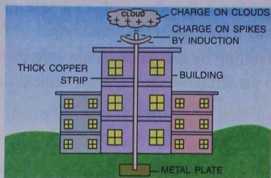
Fig. 10.19 Lightning conductor
