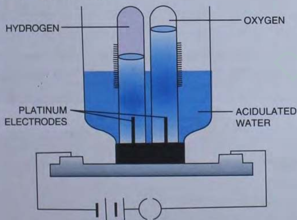
Fig. 2.1 Electrolysis of water.
