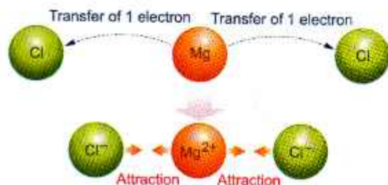
Fig. 4.14 The formation of \text{MgCl}_2
