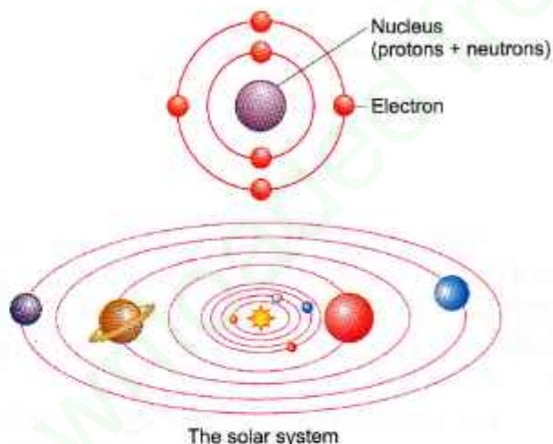
Fig. 4.8 Electrons revolve round the nucleus like planets round the sun.
