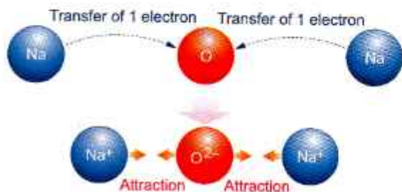
Fig. 4.15 The formation of \text{Na}_2\text{O}
