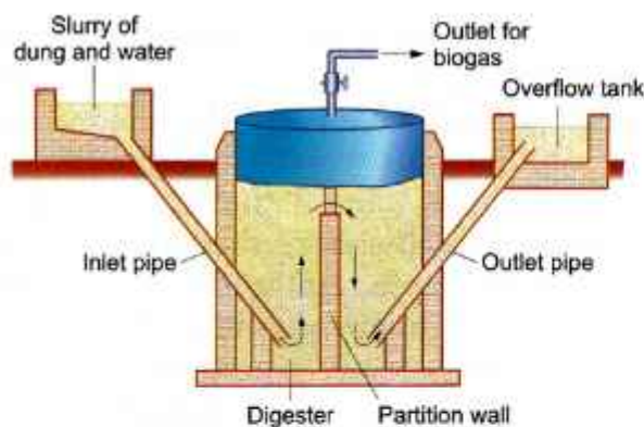
Fig. 3.3 Floating-dome biogas plant
