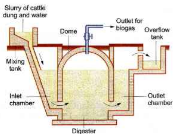
Fig. 3.4 Fixed-dome biogas plant
