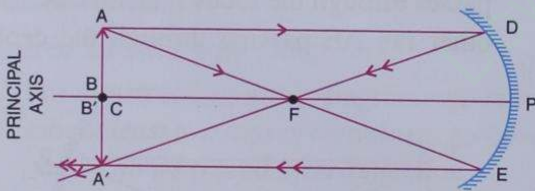
Fig. 7.13 A real, inverted image of the same size is formed at the centre of curvature
