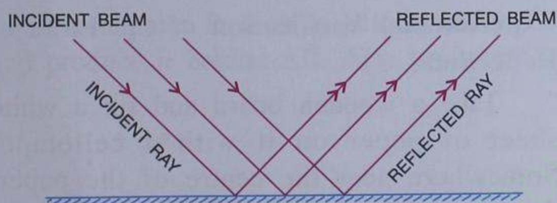
Fig. 6.2 Regular reflection
