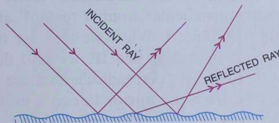
Fig. 6.3 Irregular reflection
