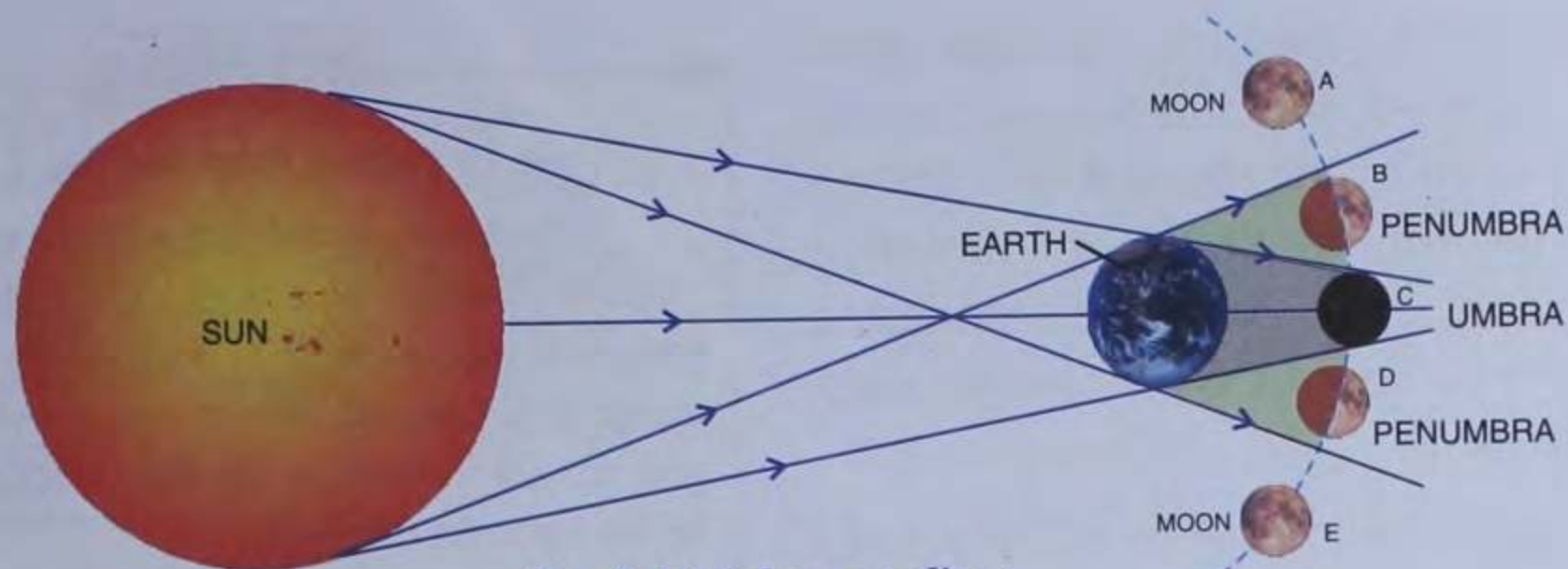
Fig. 5.14 A lunar eclipse
