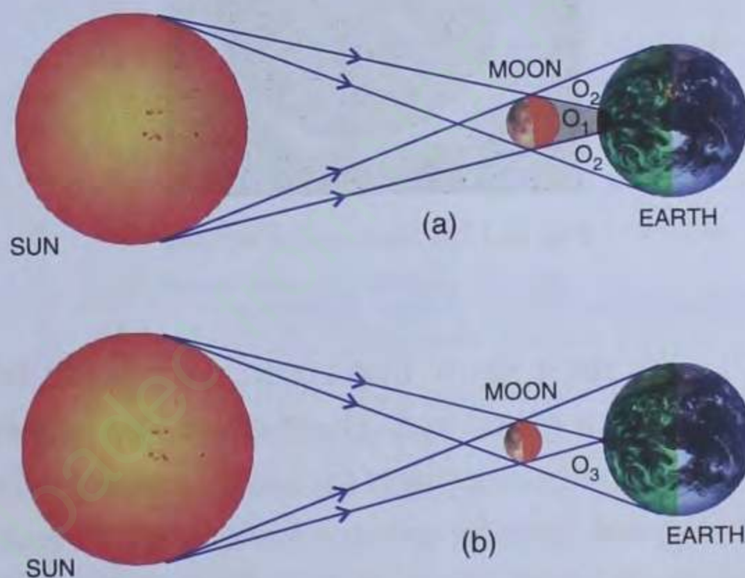
Fig. 5.16 Occurrence of different types of solar eclipses
