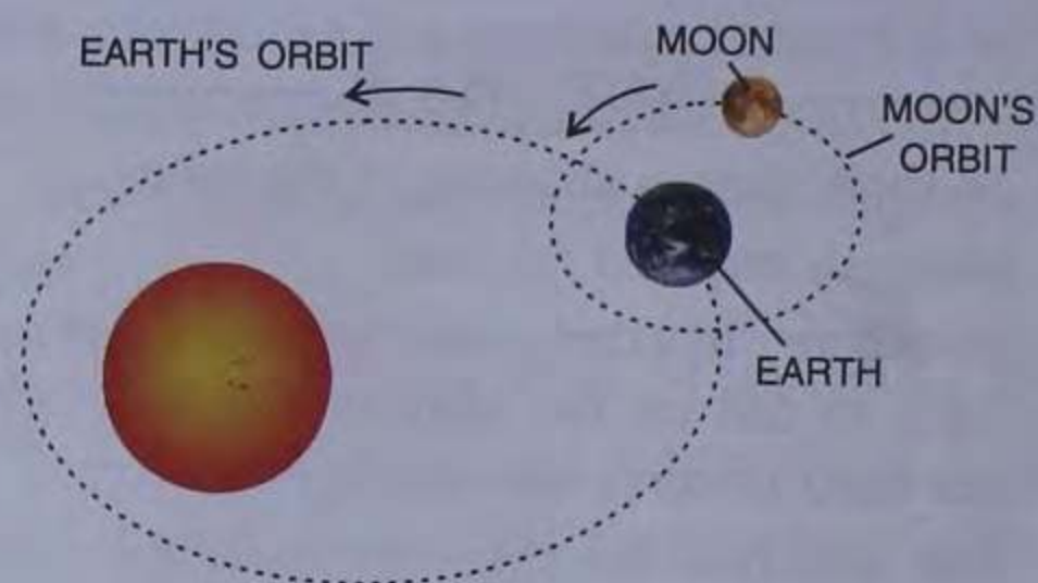
Fig. 5.13 The Earth's and the Moon's orbits
