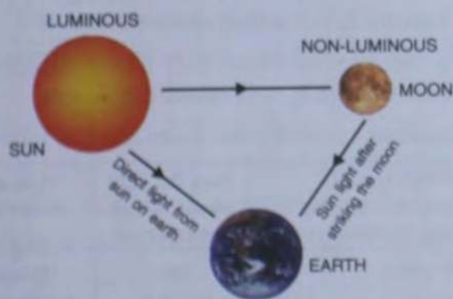
Fig. 5.5 The moon is a non-luminous body
