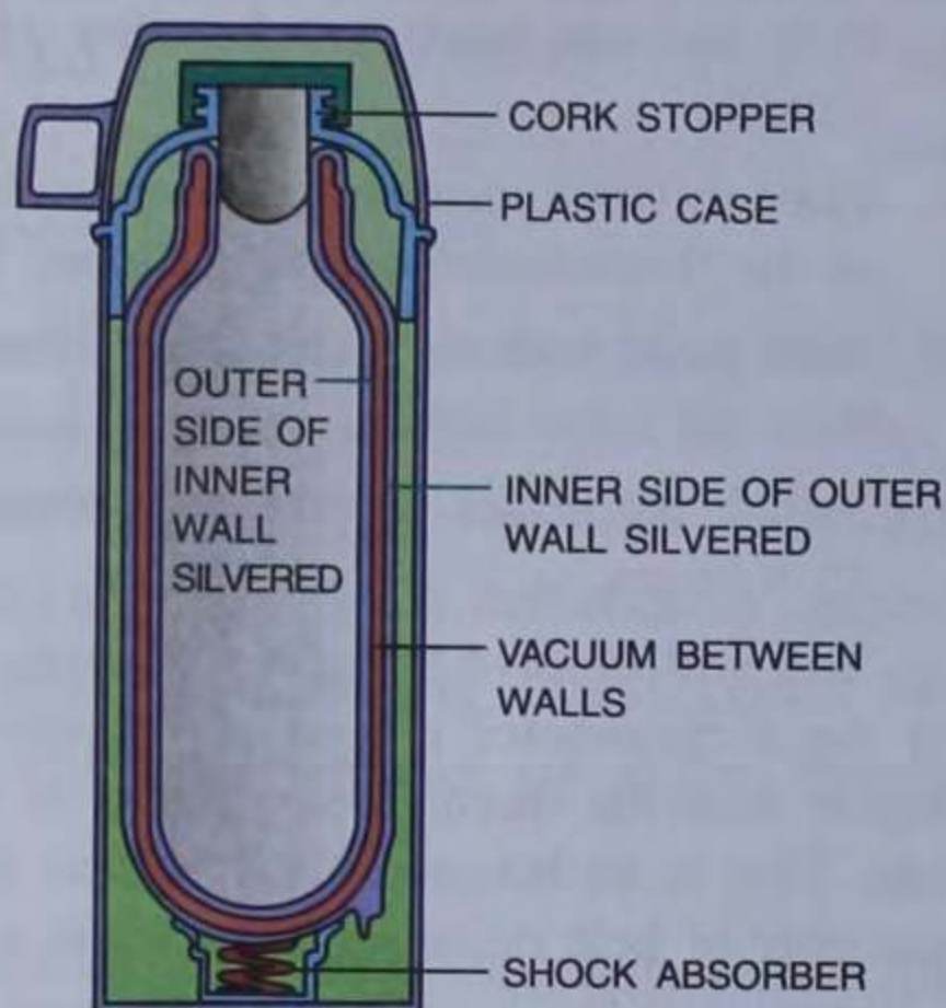
Fig. 4.26 Thermos flask
