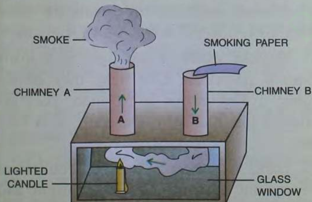
Fig. 4.23 An experiment to show convection in gases
