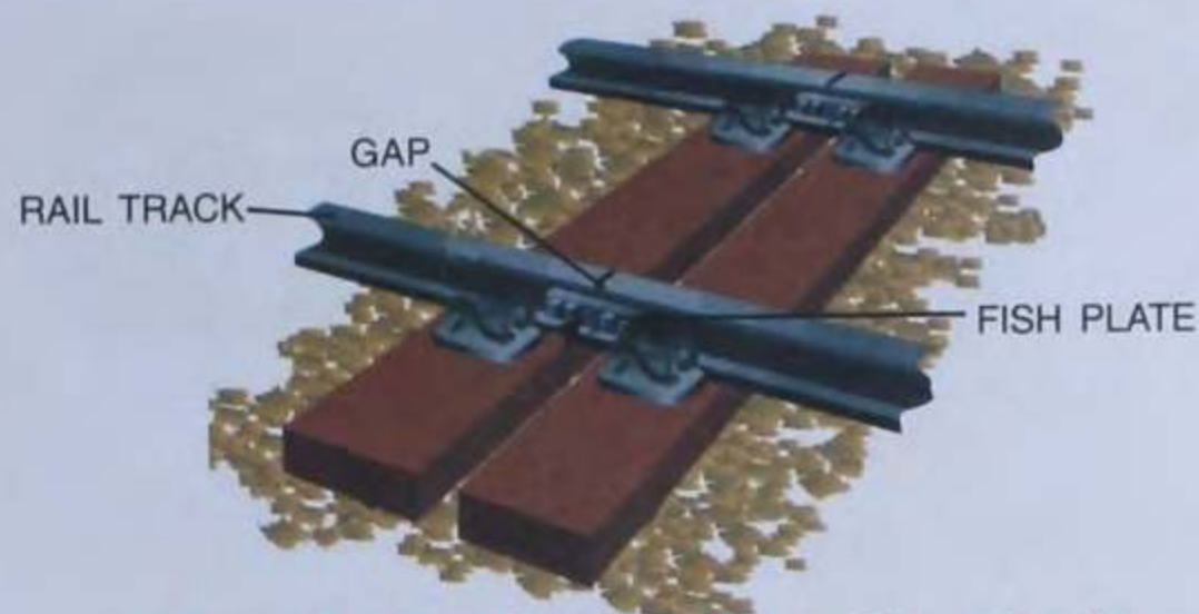
Fig. 4.13 Gap between the railway tracks
