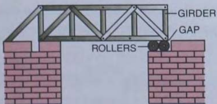
Fig. 4.12 Gap for the expansion in a bridge
