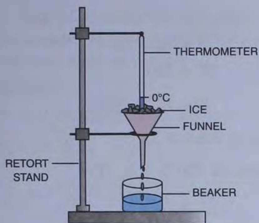
Fig. 4.5 Lower fixed point
