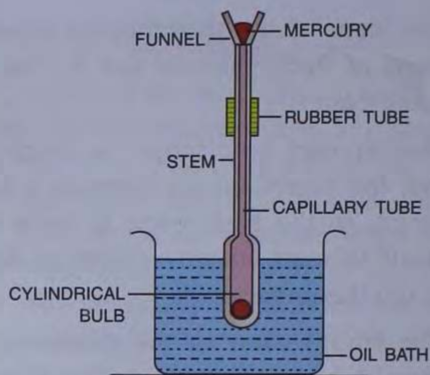
Fig. 4.4 The capillary tube being filled with mercury
