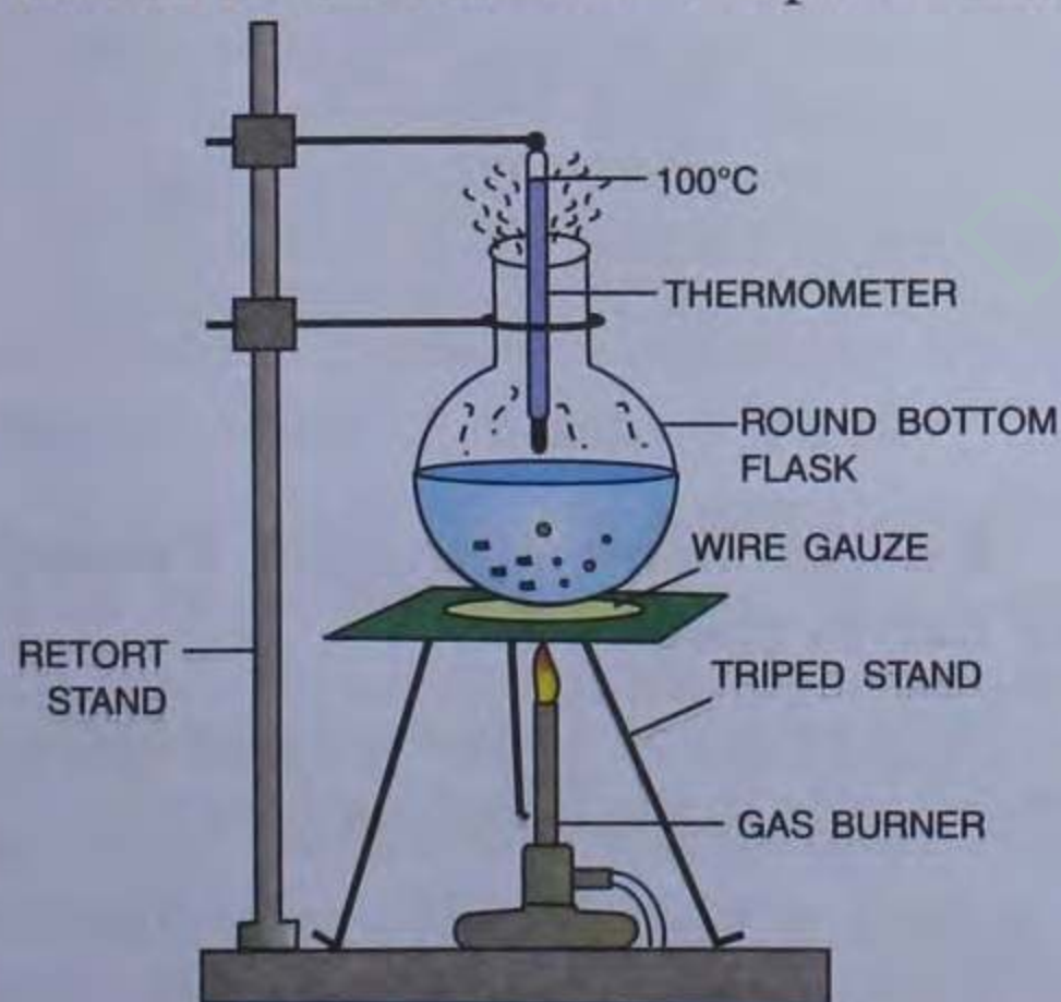
Fig. 4.6 Upper fixed point
