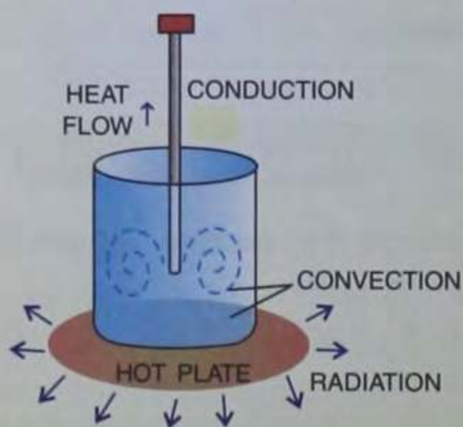
Fig. 4.19 An experiment to show how heat travels in different mediums
