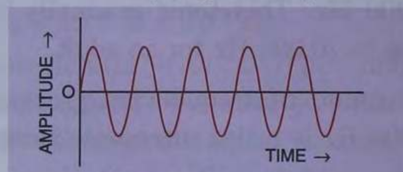
Wave with higher frequency, (High pitch sound)
