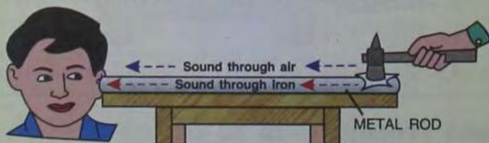
Fig. 3.11 Sound travels faster through a solid medium than through air
