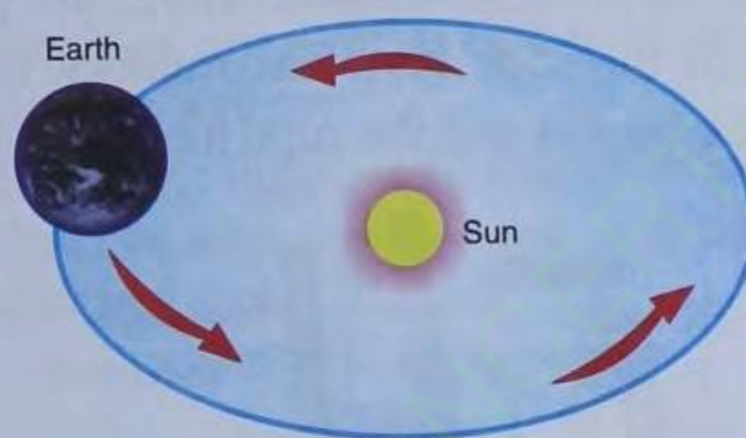
Fig. 2.8 Earth revolving around the sun
