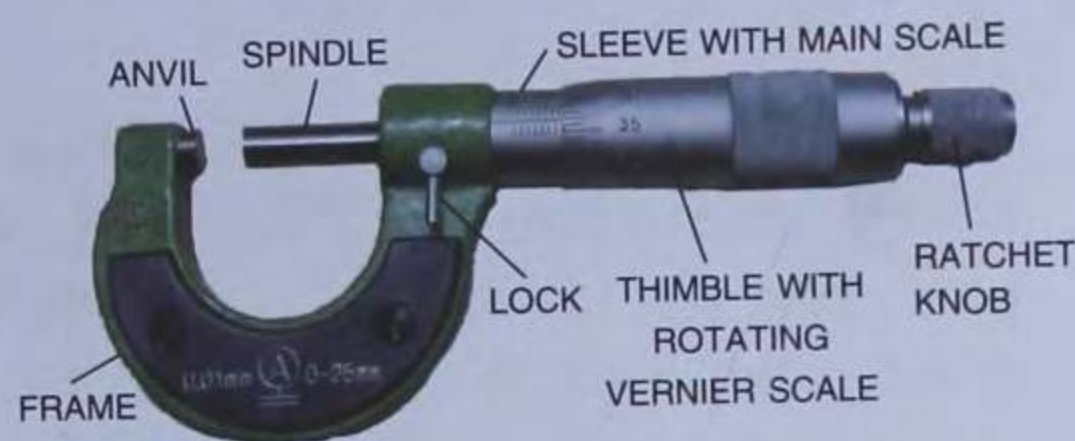
Fig. 1.10 Screw gauge
