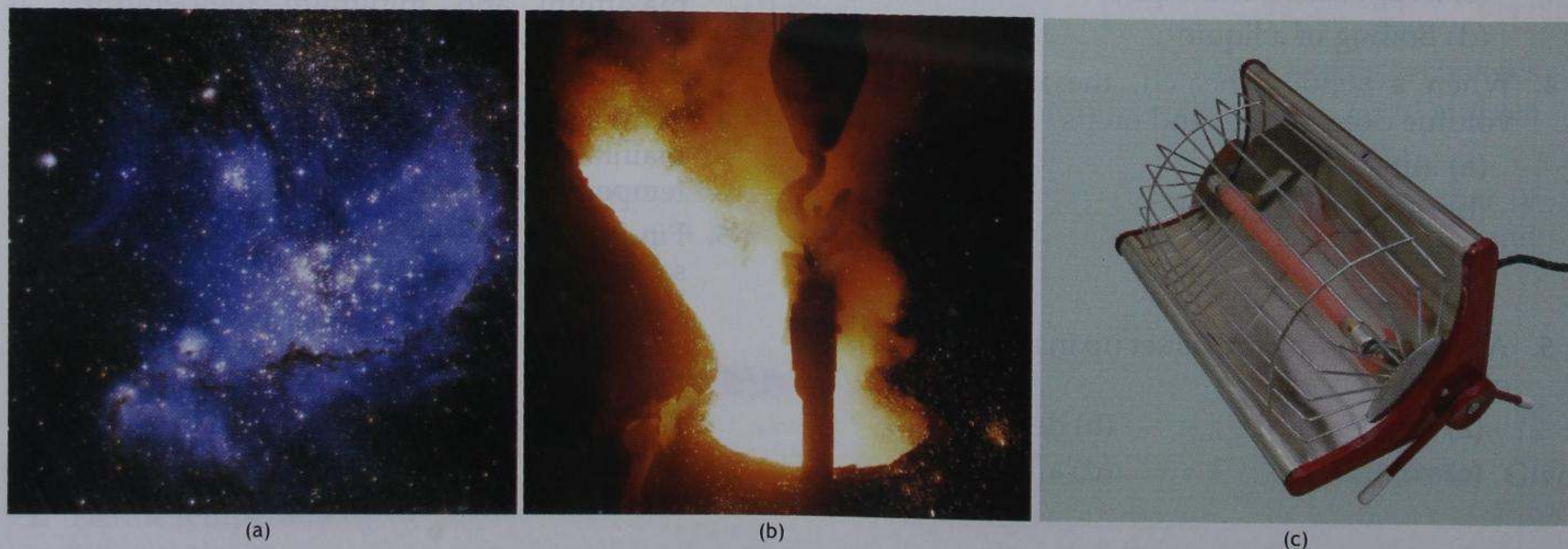
Fig. 5.1 Light is emitted by (a) the hot gases of stars, (b) molten iron and (c) the glowing coil of a heater.
