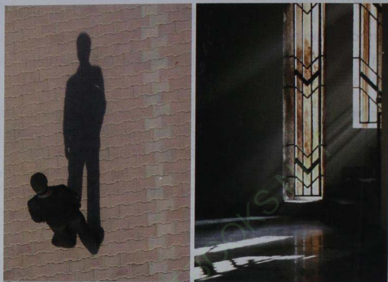
Fig. 5.7 Usually, we see a shadow when it falls on a surface. Sometimes we can also see the shadow before it falls on a surface.
