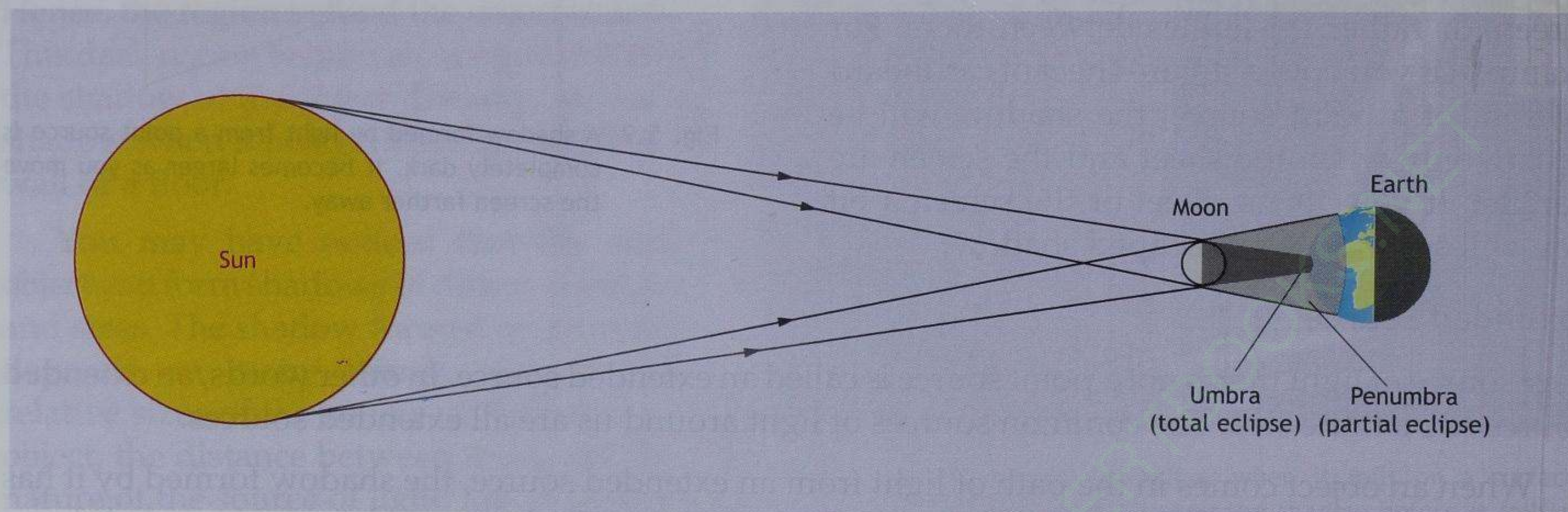
Fig. 5.11 A solar eclipse can occur only on the day of a new moon.
