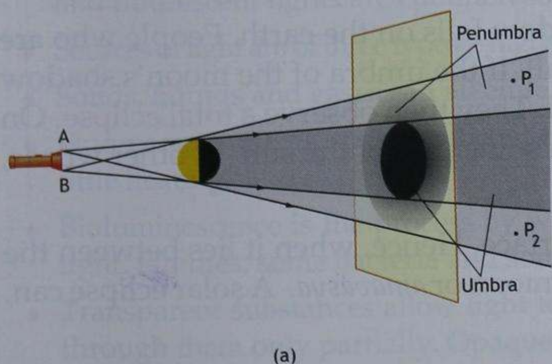
Fig. 5.10 (a) The umbra extends indefinitely when the object is larger than the source. (b) The umbra is a cone that extends only up to a particular distance when the object is smaller than the source.
