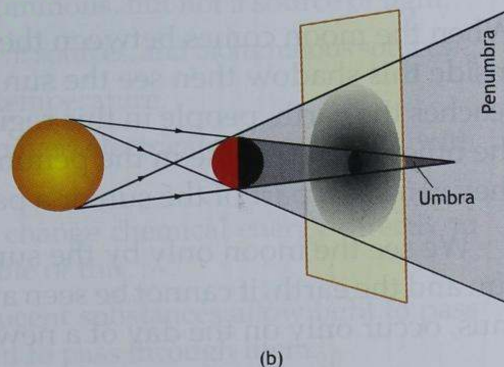
Fig. 5.10 (a) The umbra extends indefinitely when the object is larger than the source. (b) The umbra is a cone that extends only up to a particular distance when the object is smaller than the source.
