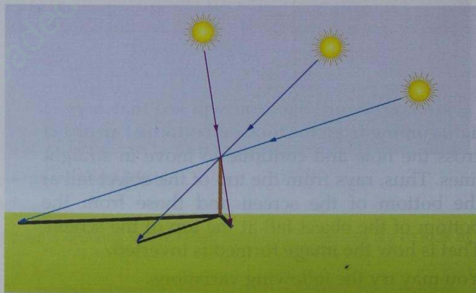
Fig. 5.8 The length of the shadow changes with the angle between the rays of the sun and the stick.
