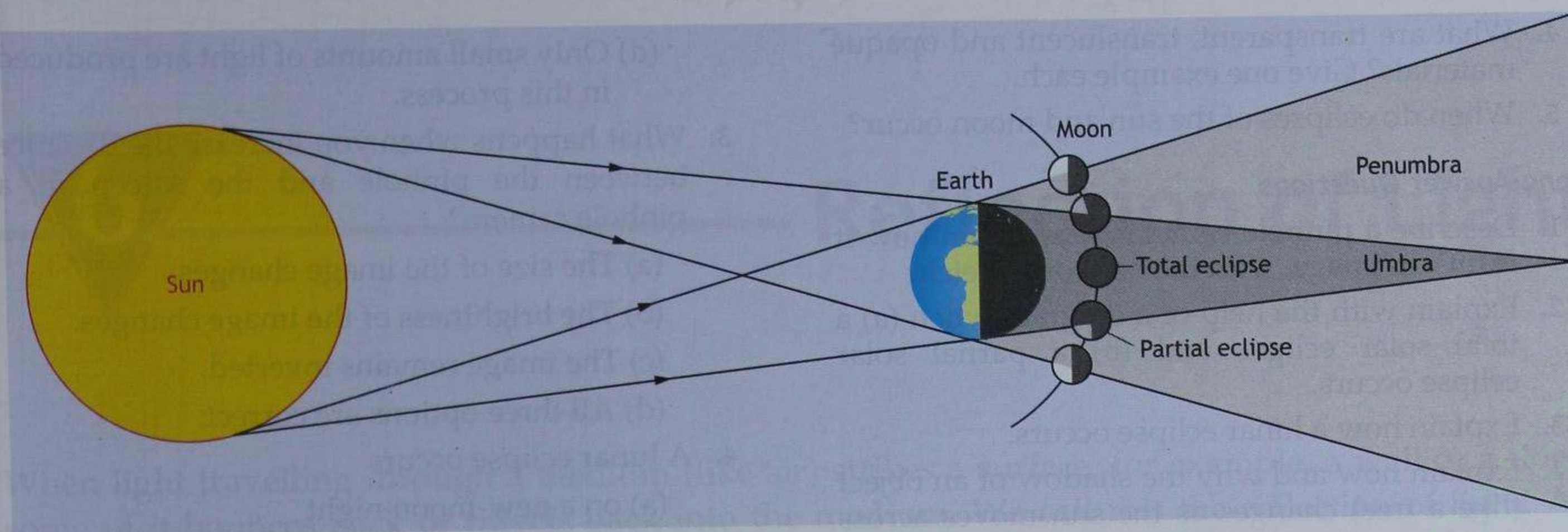
Fig. 5.13 A total lunar eclipse occurs when the moon passes through the umbra of the earth's shadow.
