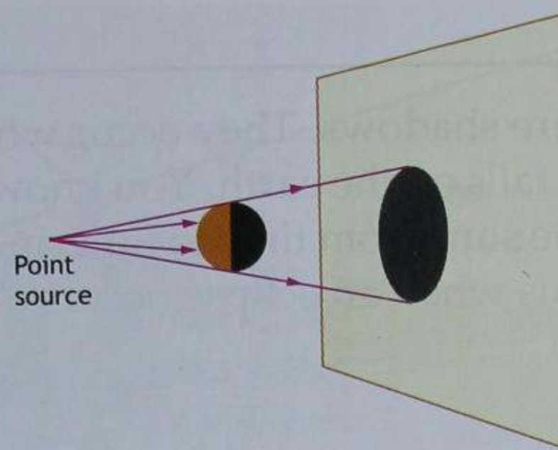
Fig. 5.9 A shadow formed by light from a point source is completely dark. It becomes larger as you move the screen farther away.
