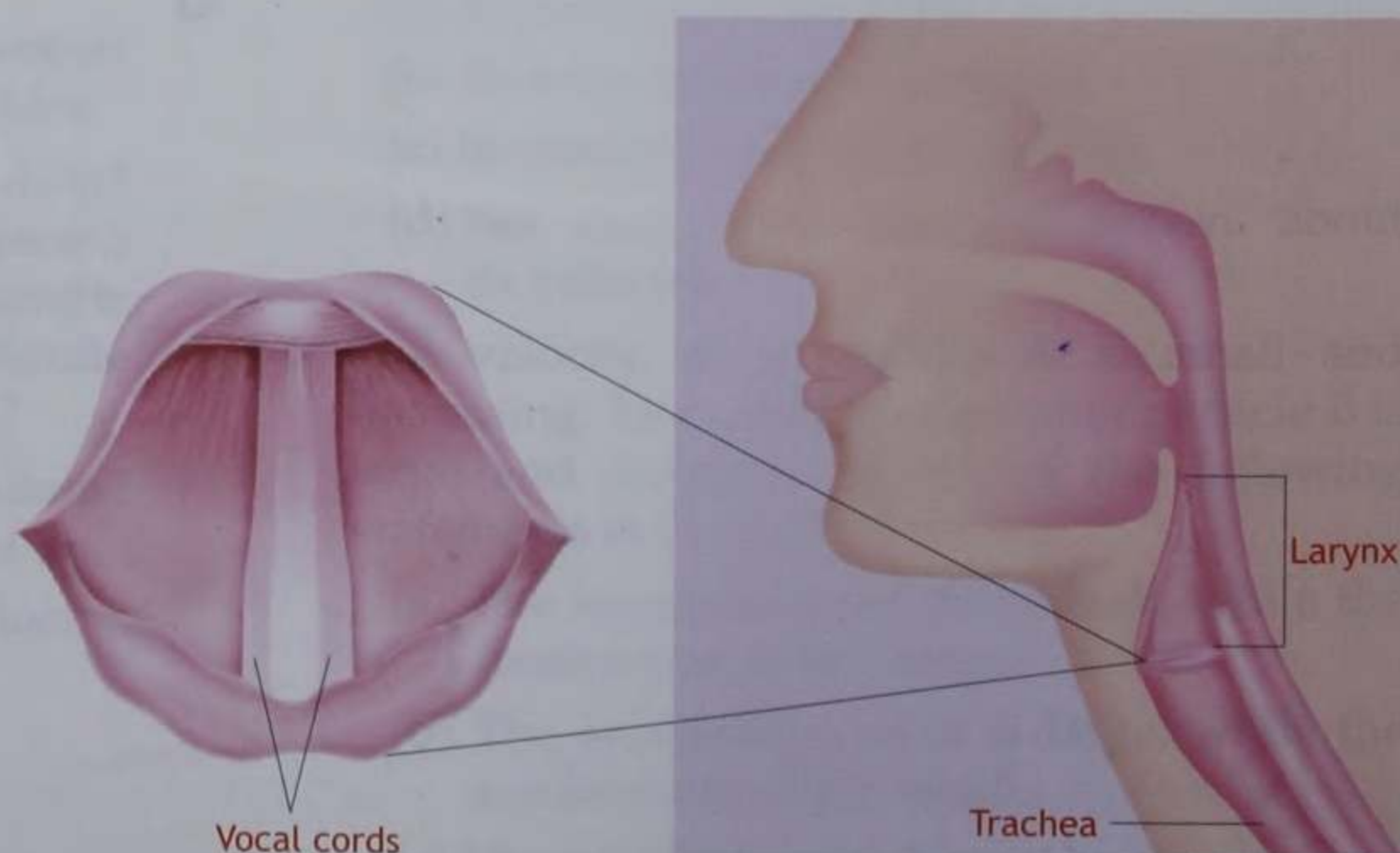
Fig. 3.2 Human larynx
