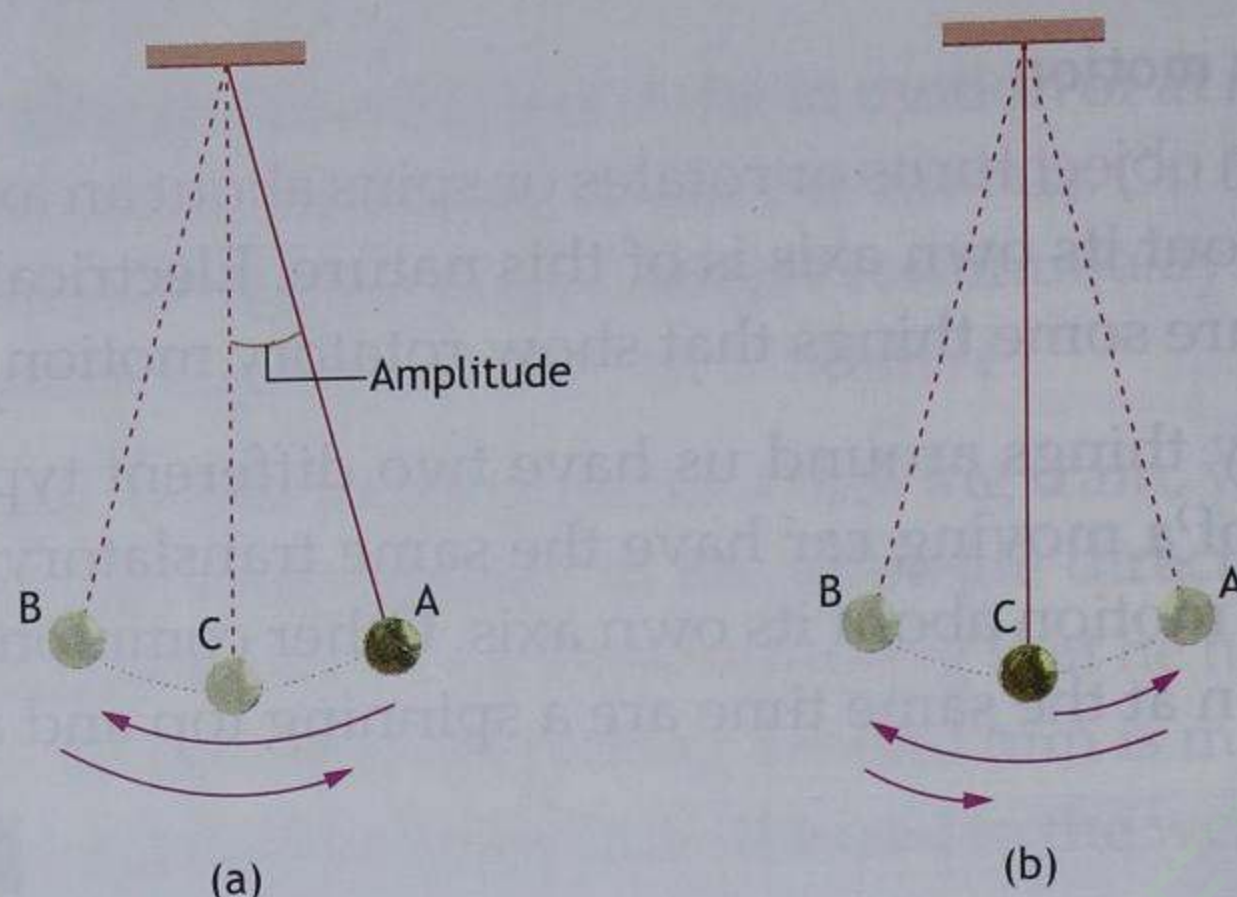
Fig. 2.5 One oscillation of a pendulum is its motion (a) from A to B and back to A or (b) from C to A to B to C.
