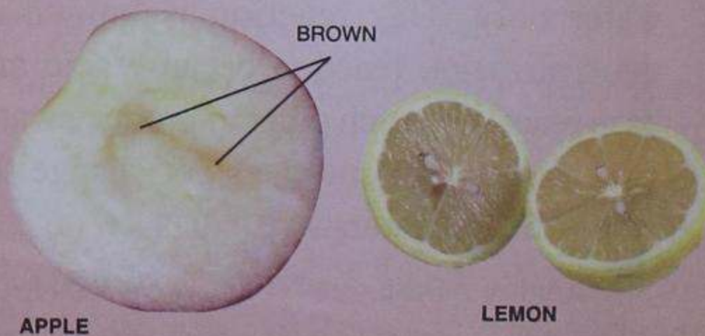
Fig. 6.7 : A piece of apple turning brown.
