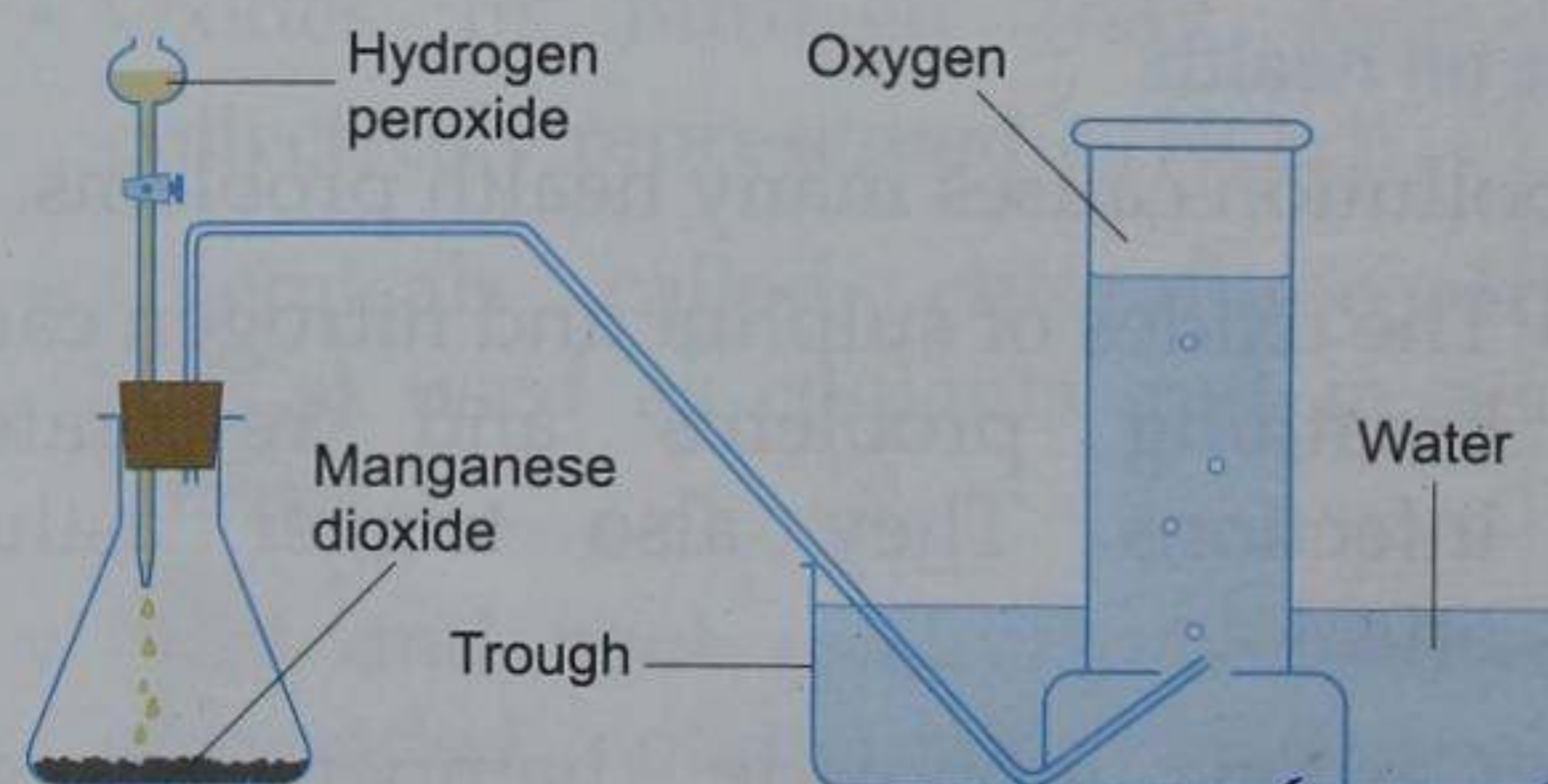
Fig. 4.1 The preparation of oxygen
