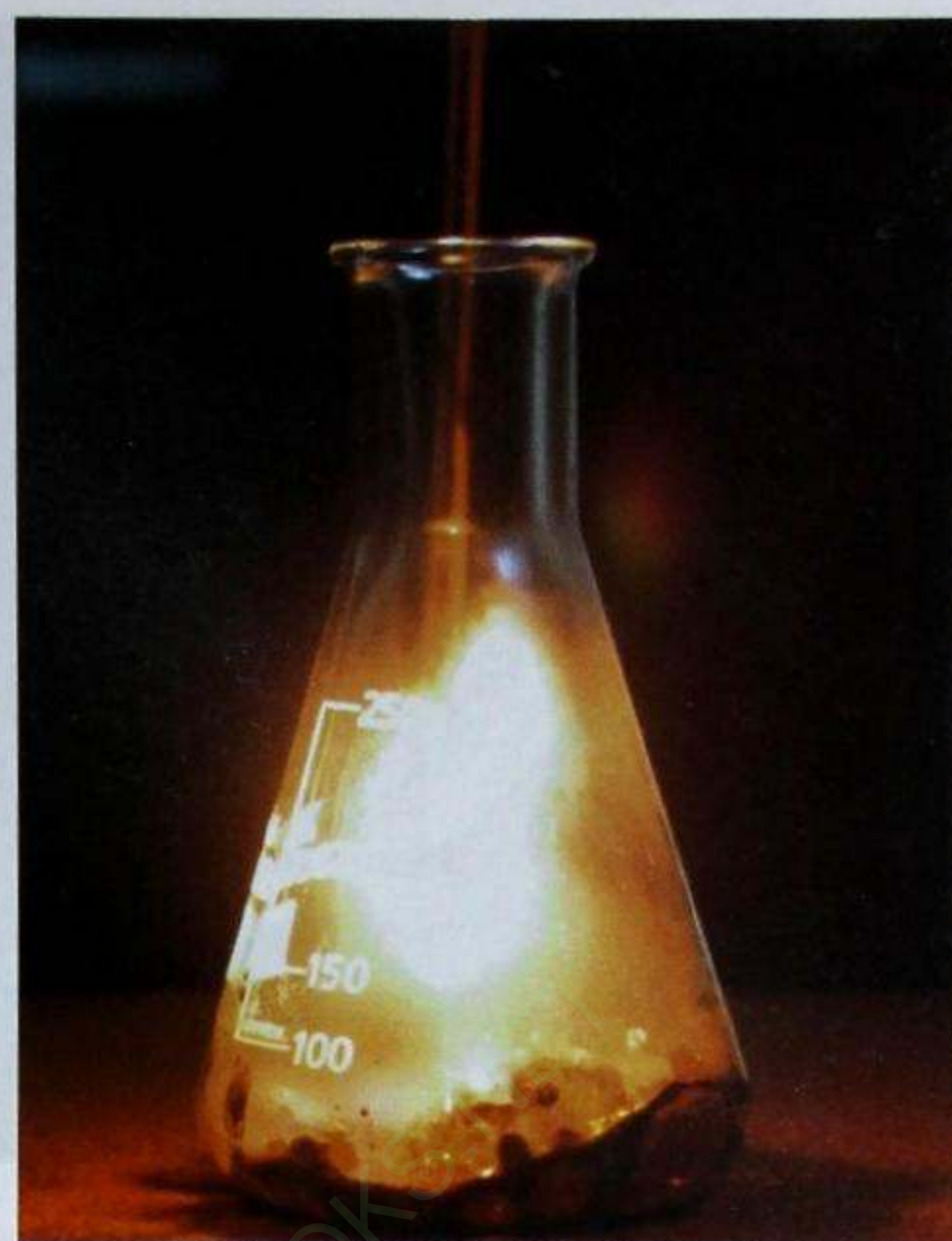
Fig. 4.5 A glowing splinter burns brightly in oxygen.
