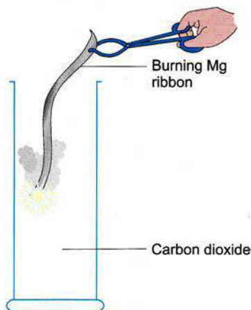
Fig. 4.10 A burning piece of magnesium continues to burn in carbon dioxide.
