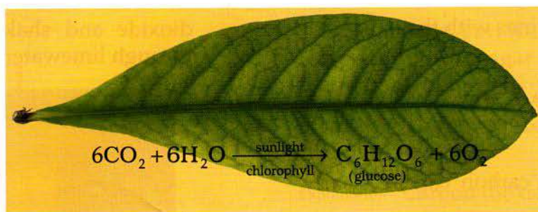
Fig. 4.8 The liberation of oxygen in photosynthesis
