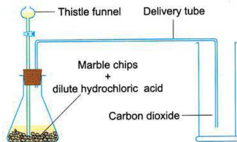
Fig. 4.9 Preparation of carbon dioxide
