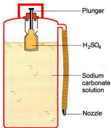
Fig. 4.12 A fire extinguisher
