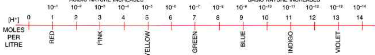
Fig. 3.2 Colour changes in the universal indicator (for different pH values).
