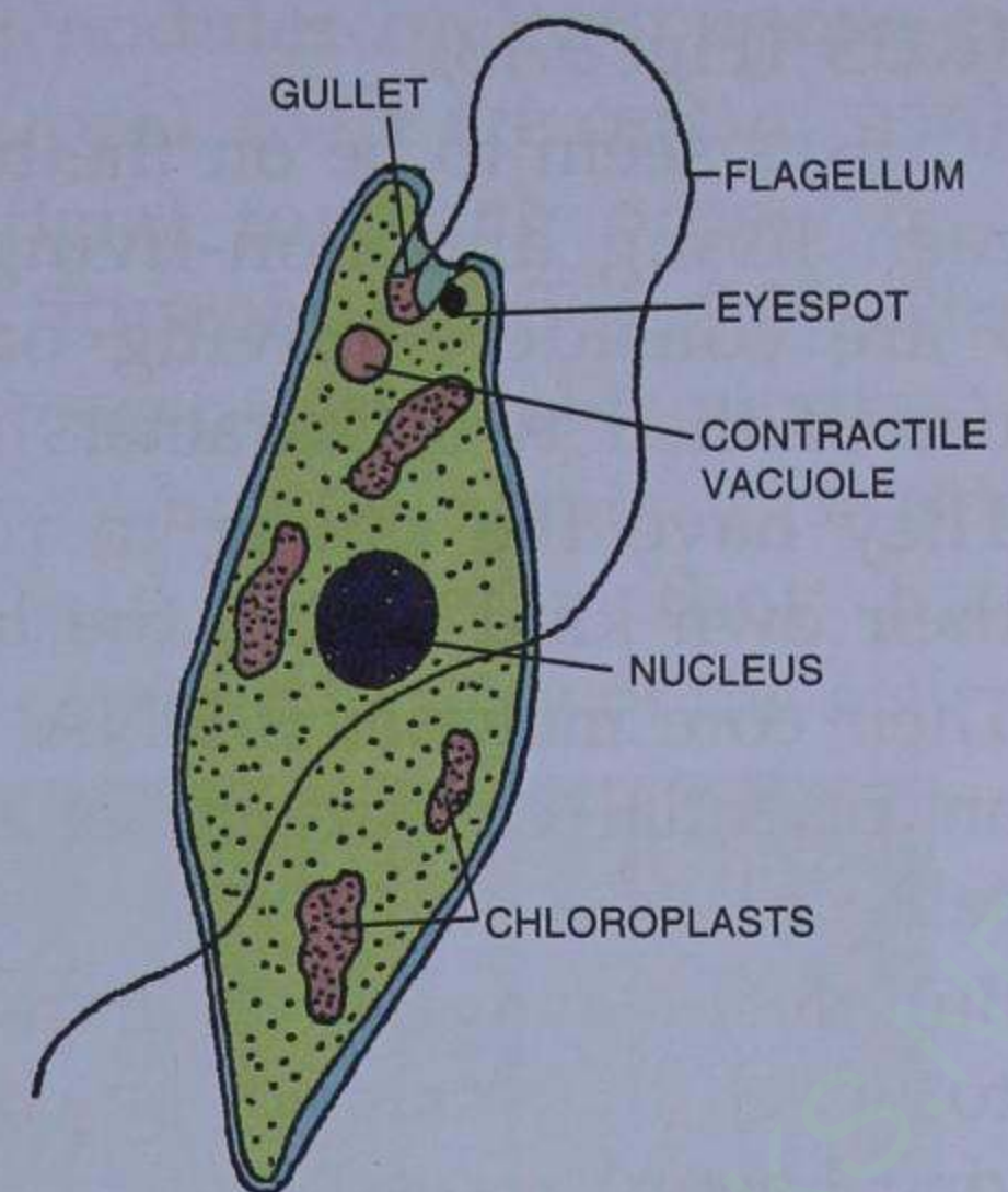
Fig. 9.16 Euglena (A plant like micro-organism) under plants. It usually reproduces by longitudinal binary fission.
