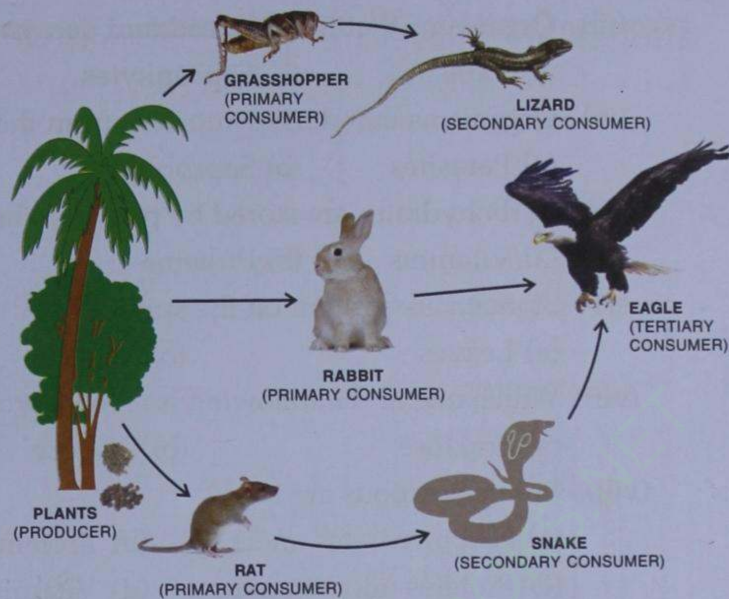
Fig. 4.8 Food chains
