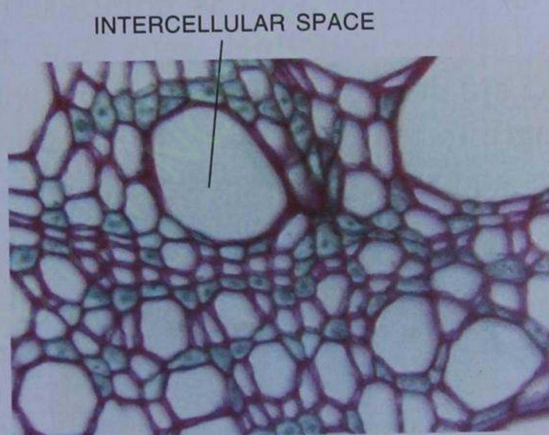
Fig. 2.6 Parenchyma cells
