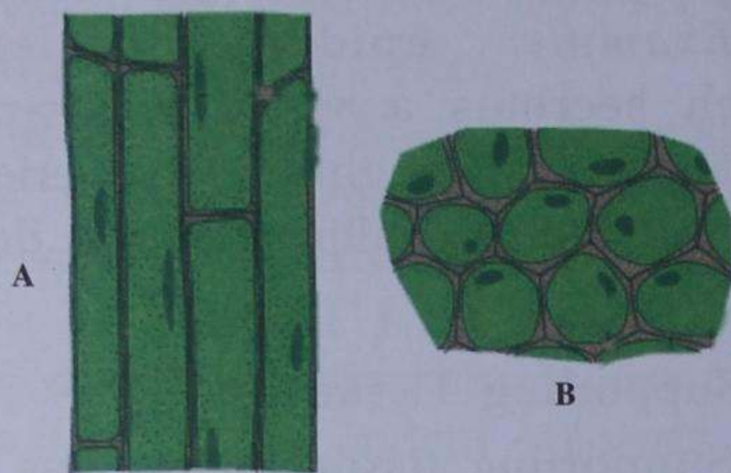
Fig. 2.7 Collenchyma
