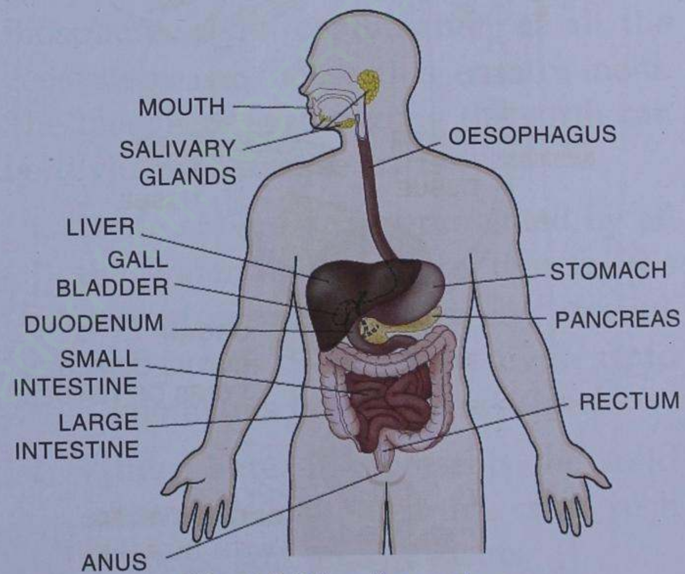
Fig. 2.2 Digestive system
