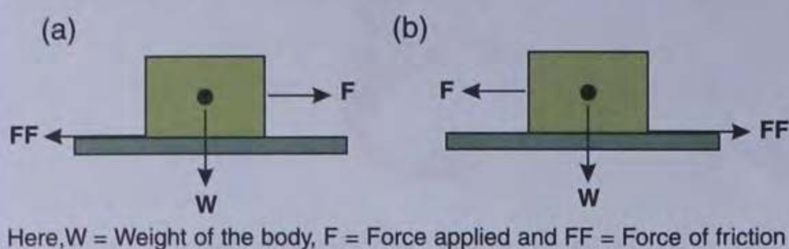
Fig. 3.2 Showing that friction always opposes the relative motion between the two bodies irrespective of the direction of motion.
