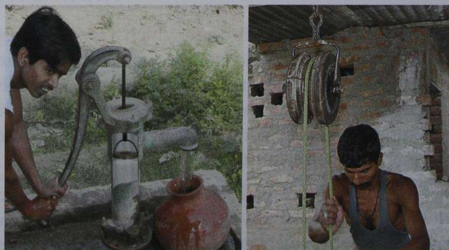
Fig. 5.3 The handle of a hand pump and a pulley change the direction in which force is applied.
