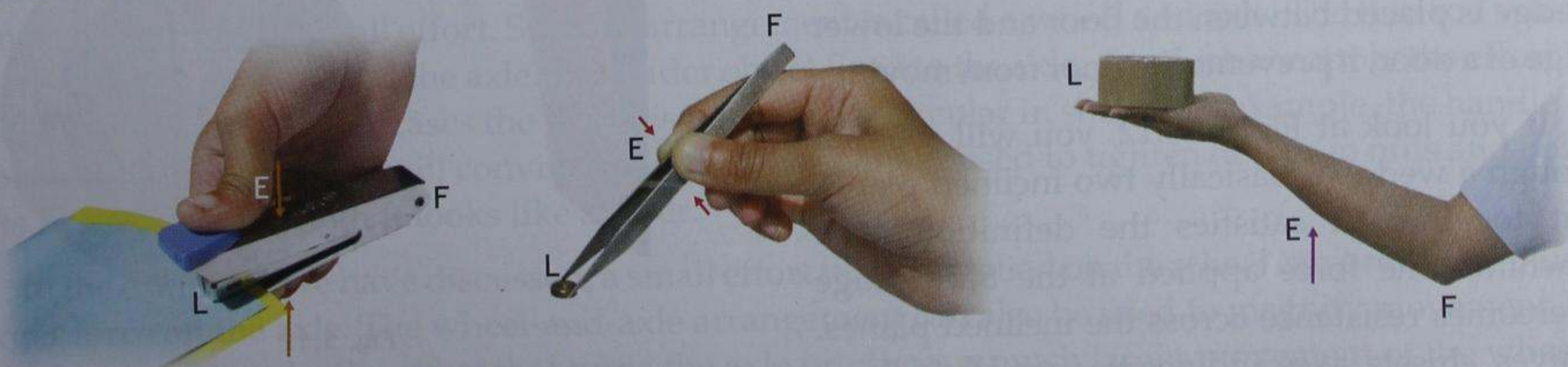
Fig. 5.10 Class-three levers
