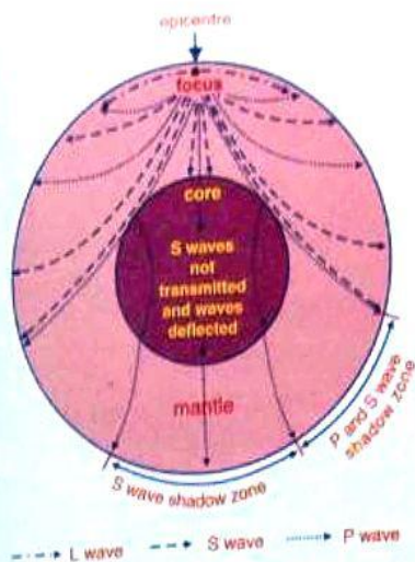
Fig. 8.3. Earthquake waves
