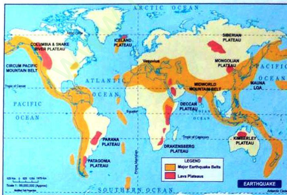
Fig. 8.1. Distribution of Earthquake belts
