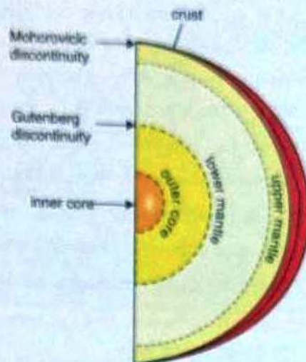
Fig. 4.5. Structure of Earth
