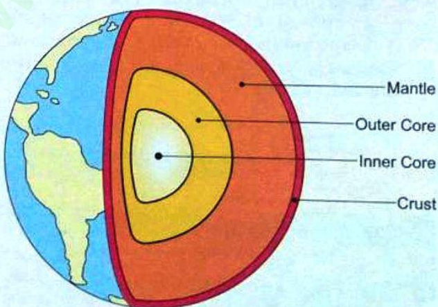
Fig. 4.1. Structure of the Earth
