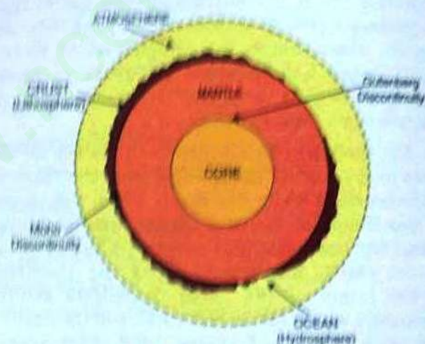
Fig. 4.4: Layers of the Earth
