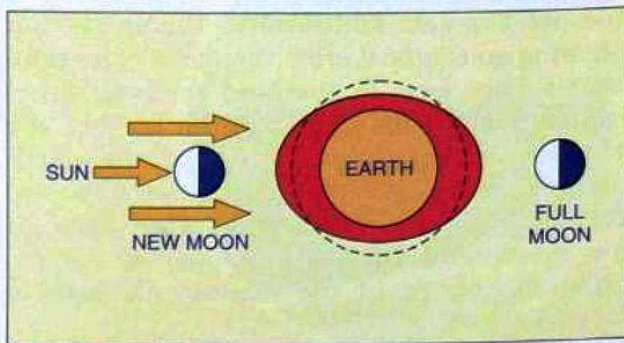
Fig. 11.4. Full moon and new moon and high tides
