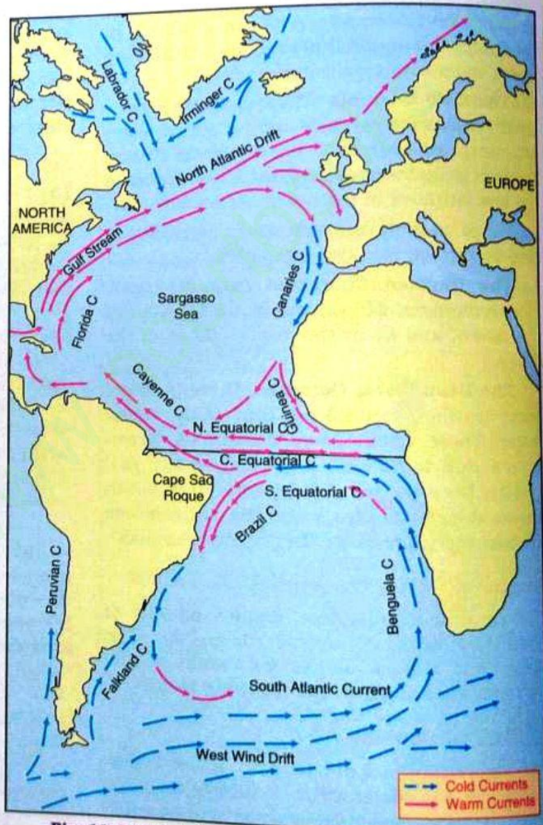
Fig. 11.6. Circulation of Currents in the Atlantic Ocean
