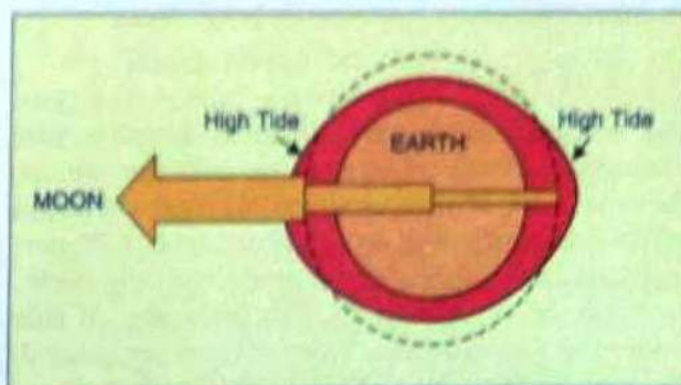
Fig. 11.3. Occurrence of high and low tides due to gravitational forces of the moon on the earth's water surface
