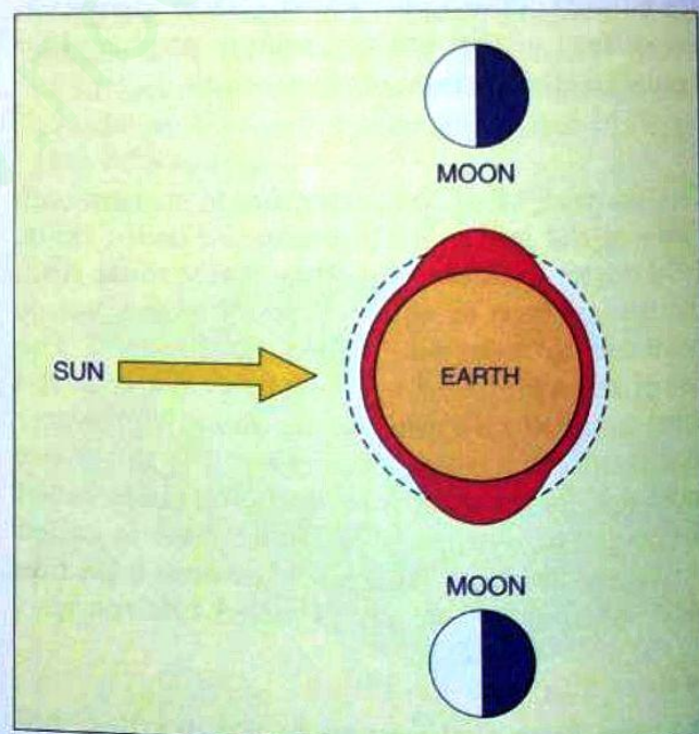
Fig. 11.5. Quadrature and low tide
