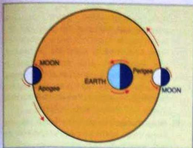
Fig. 11.2. Varying distances of the earth and moon
