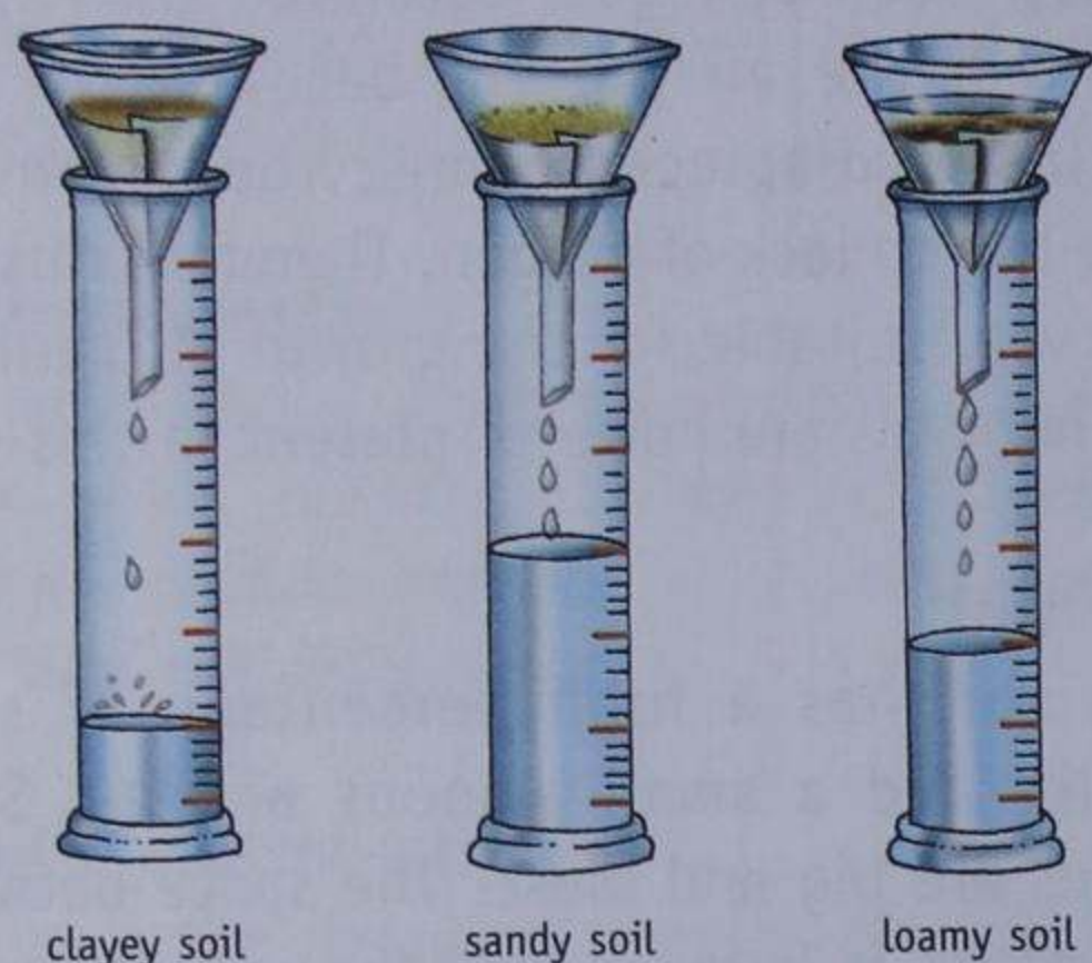
Fig. 6.8 To show the water-retaining capacity of clayey, sandy and loamy soil
