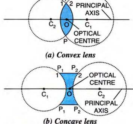
Fig. 5.7 Centre of curvature, principal axis and optical centre
