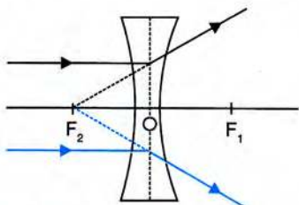
Fig. 5.37 Ray diagram for image formation by a concave lens when the object is at infinity
