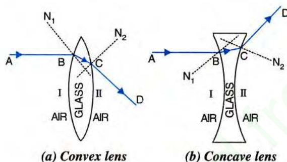
Fig. 5.14 Refraction through a lens
