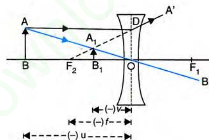
(b) Concave lens
