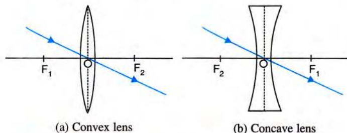
Fig. 5.19 A ray through the optiocenter passes undeviated
