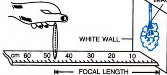
Fig. 5.57 Determination of focal length of a convex lens by the distant object method
