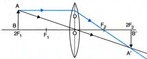
Fig. 5.33 Image formation by a convex lens for the object at 2F_1
