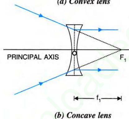
Fig. 5.10 First focus and focal length
