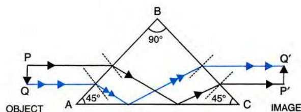
Fig. 4.49 Erecting prism
