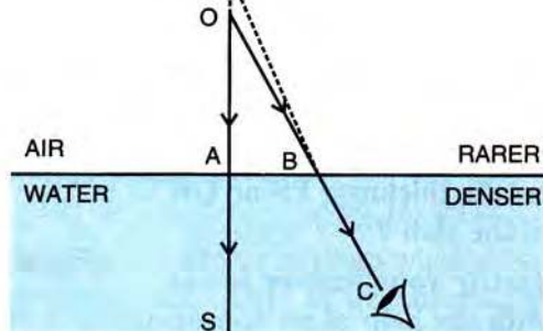
Fig. 4.38 An object in rarer medium viewed from a denser medium
