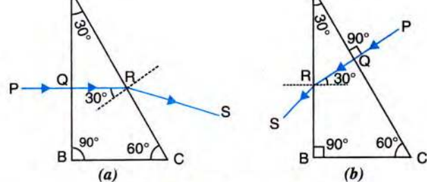
Fig. 4.52 No total internal reflection through a 30^\circ, 90^\circ, 60^\circ prism
