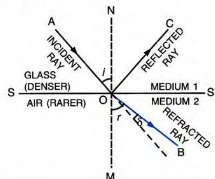
Fig. 4.2 Refraction from denser to rarer medium
