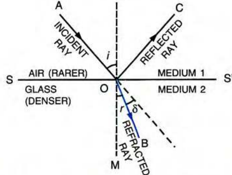
Fig. 4.1 Refraction from rarer to denser medium
