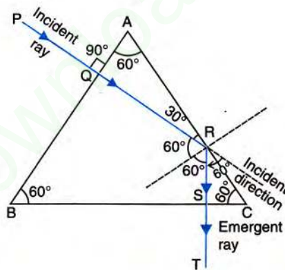
Fig. 4.50 Deviation through 60^\circ by an equilateral prism
