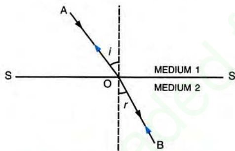
Fig. 4.5 Principle of reversibility
