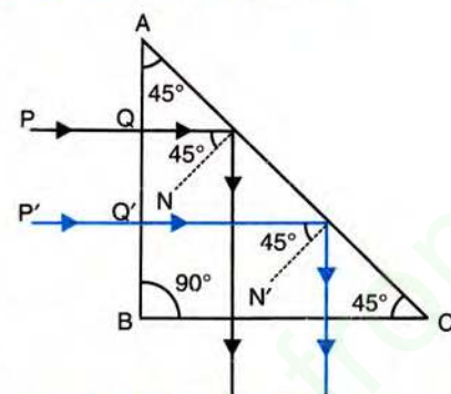
Fig. 4.47 Deviation through 90^\circ
