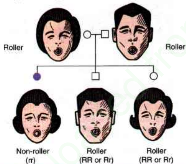
Fig. 3.3 A pedigree (family) chart showing inheritance of the ability to roll the tongue. (Symbols : O = female, □ = male; solid symbol indicates the character being traced)
