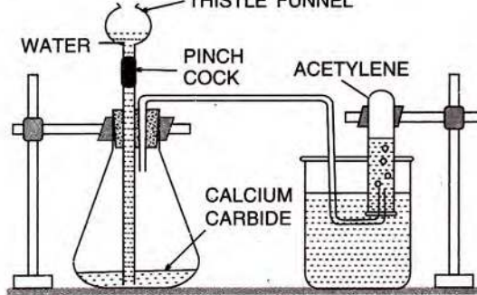
Fig. 12.5 Lab. preparation of (acetylene) ethyne.
