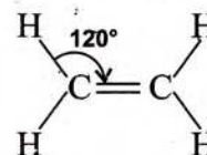
Fig. 12.3 Structure of ethylene
