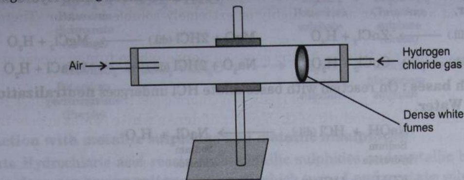
Fig. 4 : Showing Hydrogen chloride gas is heavier than air
