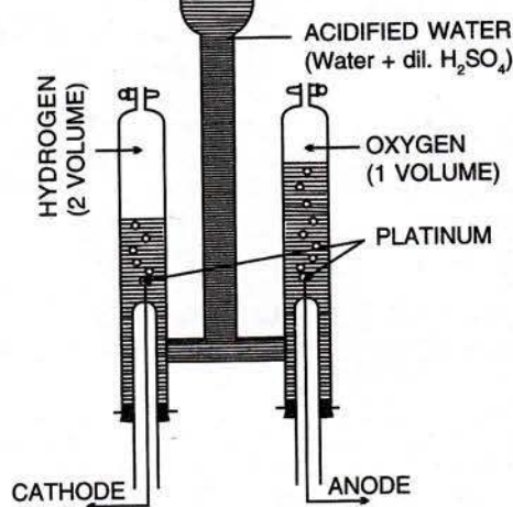
Fig. 6.5 Electrolysis of acidified water using platinum electrodes.
