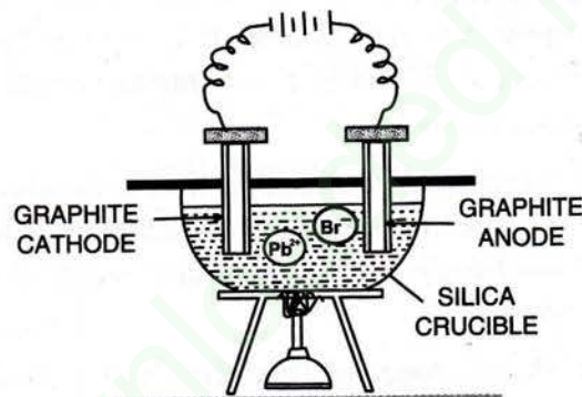
Fig. 6.4 Electrolysis of molten lead bromide.
