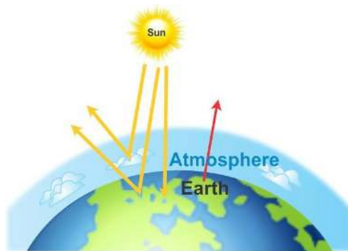
Greenhouse Effect
